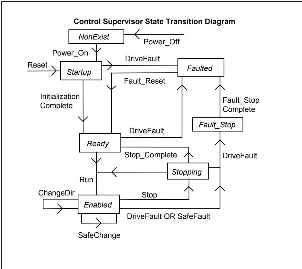
Figure 7- 2. Control Supervisor State Transition Diagram
