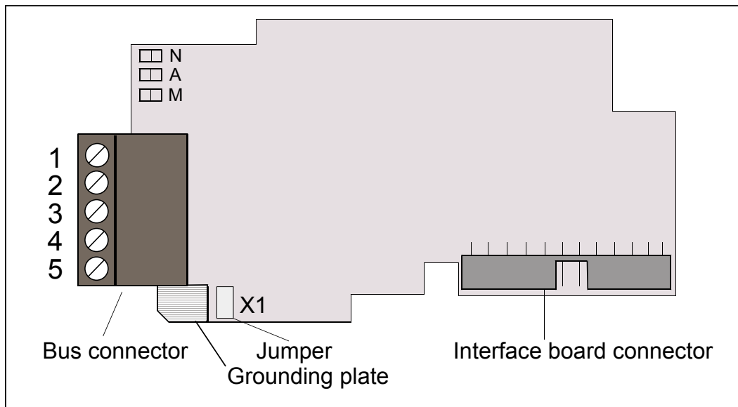
Figure 4-1. Vacon DeviceNet option board NXOPTC7
