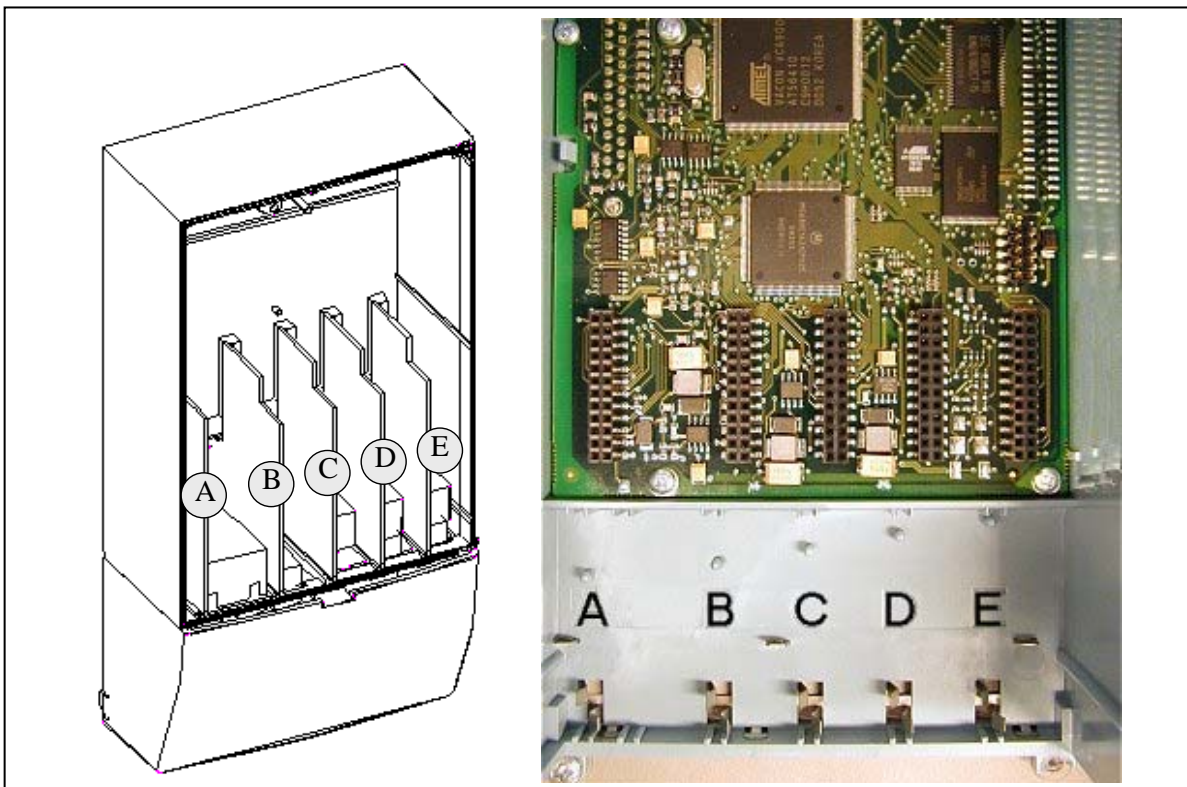
1.1 Board slots on the control board of Vacon NXS and NXP
